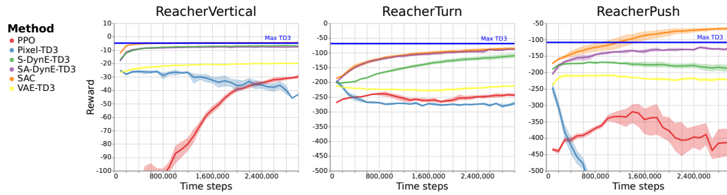
Figure 11: These plots allow for direct comparison between the methods from pixels (Pixel-TD3, VAE-TD3, S-DynE-TD3, and SA-DynE-TD3) and our baselines from low-dimensional states (PPO and SAC). The DynE methods from pixels perform competitively with some baselines from states.
