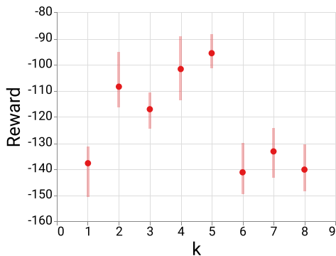
Figure 9: DynE-TD3 results on Reacher Push with varying k . We find that increased temporal abstraction improves performance up to a point, beyond which the action space is no longer able to represent the optimal policy and performance degrades. Solid points are the mean reward obtained after training for 1M environment steps. Shaded bars represent the min and max performance over 4 seeds.
